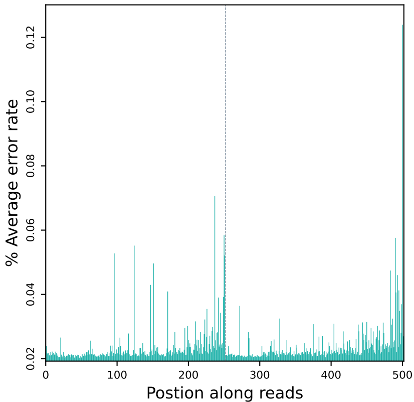
Error rate distribution along reads (R10713)
